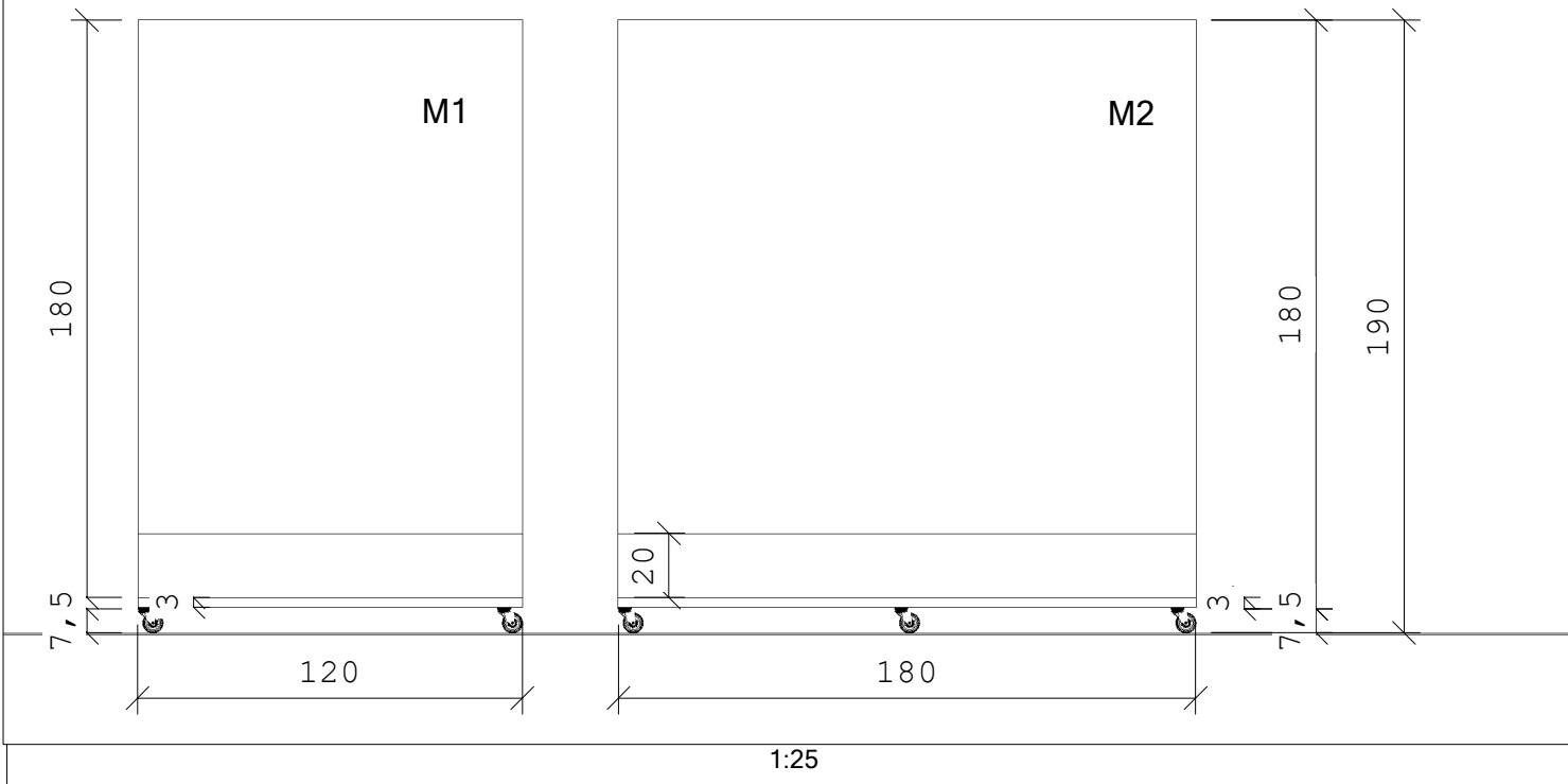
VISTA FRONTAL
